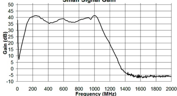
Small Signal Gain
